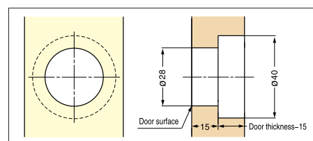
Bore Dimensions
