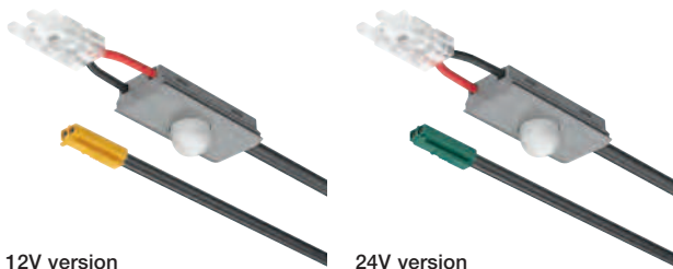
12V version
