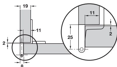
Screw mounting
