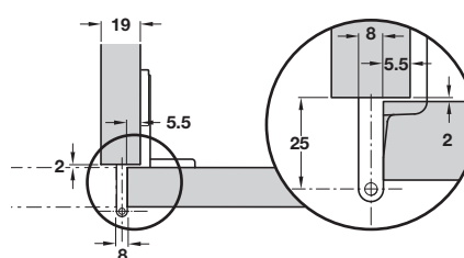
Screw mounting
